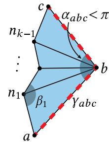
Fig. 34. Notation for FLIPOUT.
