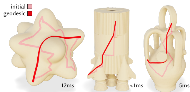
Fig. 35. Basic results shortening an initial path to a geodesic by flipping edges. Inset values give the runtimes. All of the resulting curves shown are exact polyhedral geodesics.
