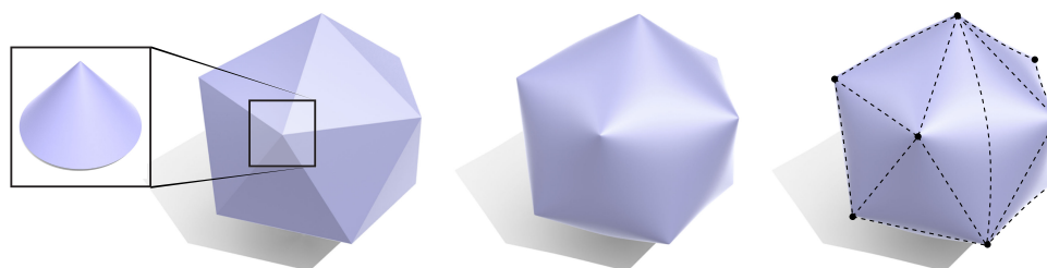
Fig. 12. Left : intrinsically, a small neighborhood around any vertex of a polyhedral surface is indistinguishable from a round circular cone. For instance, a vertex made from triangular pieces of paper can be easily smoothed out into a circular cone without stretching or ripping. Center : a good mental “cartoon” of an intrinsic triangulation is hence a surface where the edges are completely smooth, and only the vertices are visible. Right : from this perspective, no one triangulation is special—there are many intrinsic triangulations that describe the exact same geometry.
