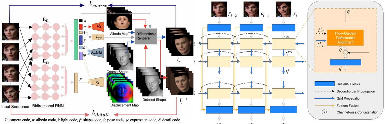
Figure 1: (Left) Our network architecture. Modified based on DECA [9], we replace DECA’s encoders with temporal encoders to encode temporal information from video sequences. (Right) Details of our bidirectional-RNN temporal feature extractors with second-order grid propagation and flow-guided deformable alignment, modified based on BasicVSR++ [5].
