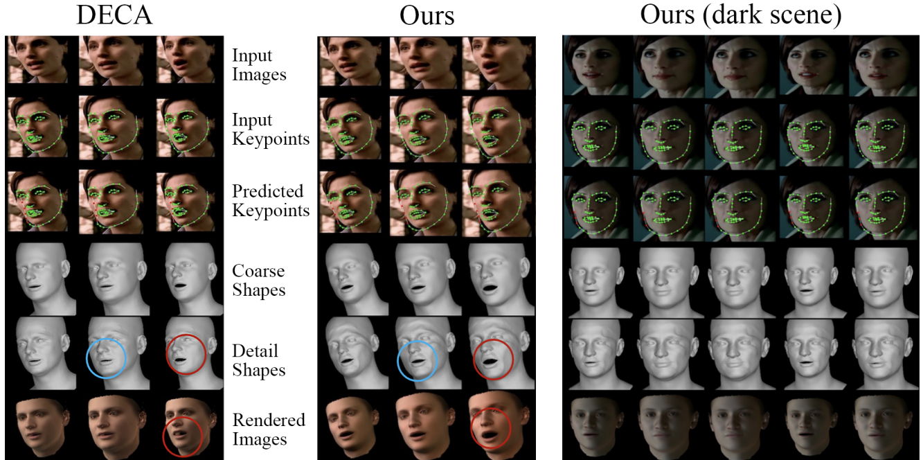
Figure 4: Qualitative evaluation results. (left) DECA v.s. our improve method with temporal encoders on a sequence from Castle in our dataset. The circles show improvements in facial expressions (especially details of mouths). Although there are still incorrect predictions for facial keypoints (see red points in row 3), they align better with the ground truths. (right) Our method on a sequence in dark scene in Castle. The facial details could still be accurate in these settings.
